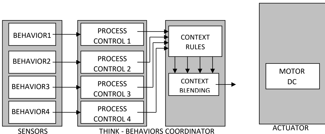
Gambar 12. Blok Diagram Behavior Based Control Architecture
